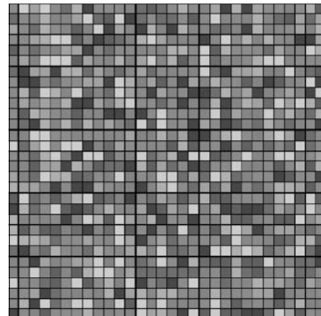
Digits of \pi represented by grey tones
