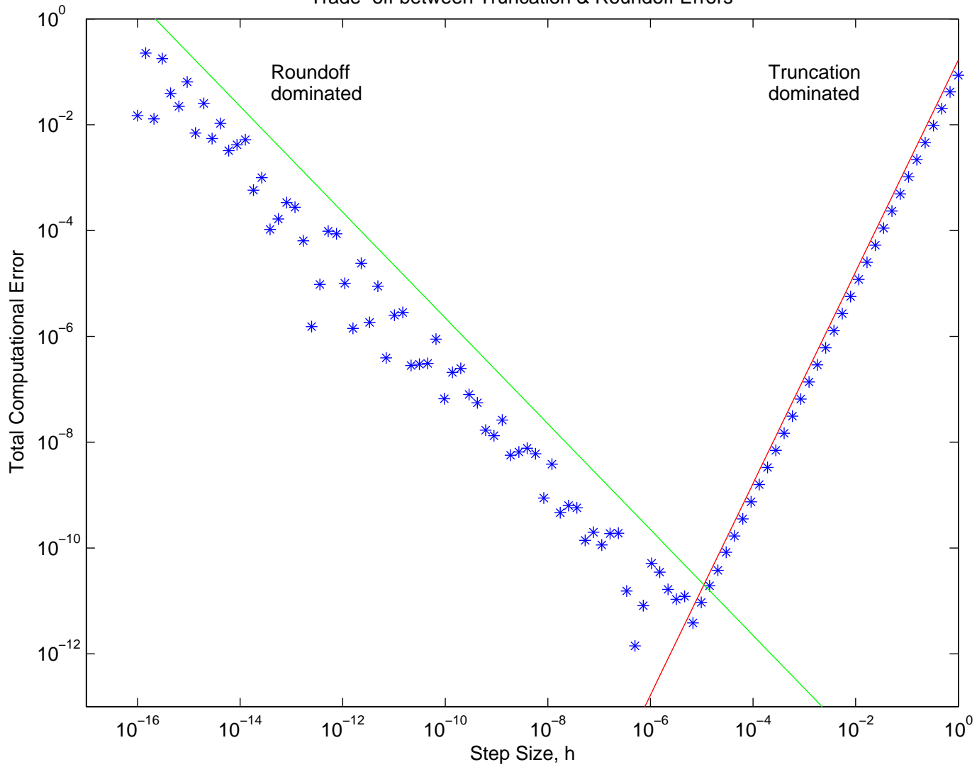
Centered Difference Formula for first derivative Trade-off between Truncation & Roundoff Errors
