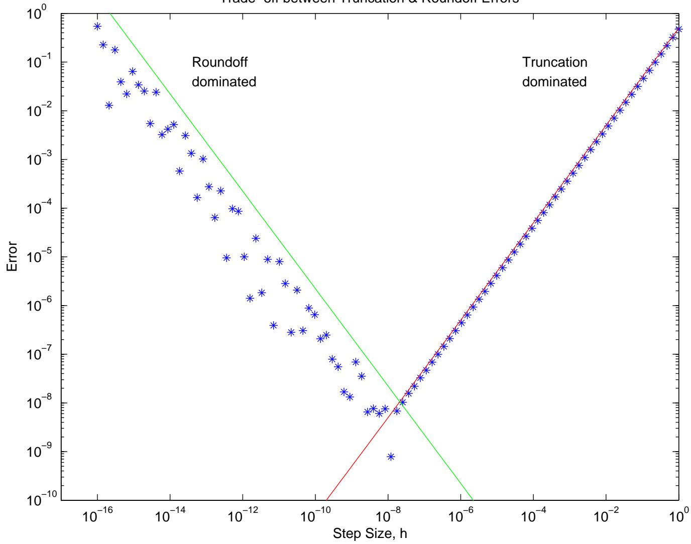
Forward Difference formula for first derivative Trade-off between Truncation & Roundoff Errors
